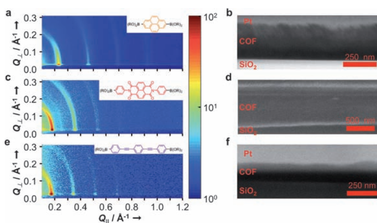
Figure 4. Grazing incidence X-ray diffraction patterns and cross-sectional SEM for a,b) ZnPc-Py COF, c,d) ZnPc-NDI COF, and e,f) ZnPc-PPE COF. The maximum intensity of each (100) Bragg peak is normalized to 100 counts.
